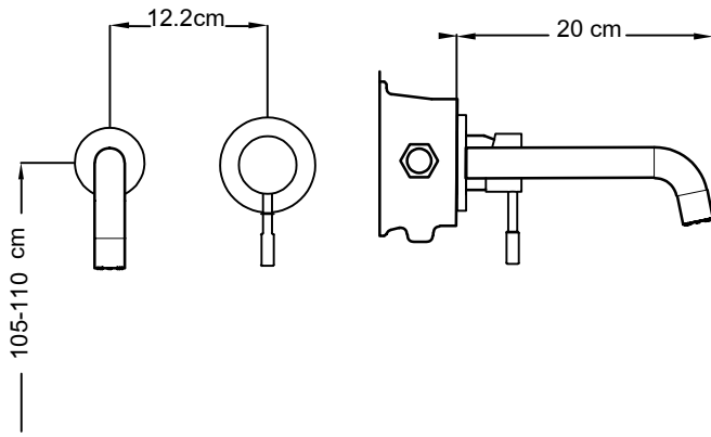
BASIN MIXER
