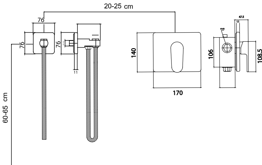
SHOWER MIXER توالی Built-in
